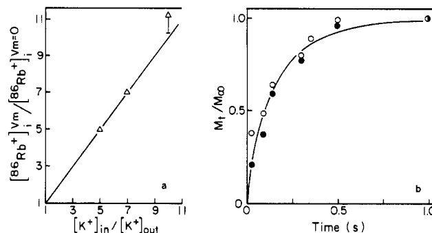
FIGURE 1: (a) Distribution of 86 Rb + according to a transmembrane voltage that was produced by the asymmetrical distribution of K + inside and outside the vesicles in the presence of valinomycin. The membrane vesicles (100 \mu g of protein/mL) equilibrated with buffer B (see Experimental Procedures) were mixed with an isotonic arginine solution (90 mM arginine chloride, 1 mM CaCl 2 , 1.5 mM sodium phosphate buffer, pH 7.0) to give a ratio of K + concentration outside to inside the vesicles as indicated on the abscissa. 86 Rb + (50 \mu Ci/mL) and valinomycin (5 \mu M) were added to the vesicle suspension for 12 s, and the reaction mixture was then applied to a Millipore filter and washed with 10 mL of buffer A (see Experimental Procedures). In control experiments ( V m = 0 mV), the vesicles were diluted with buffer B. The distribution of 86 Rb + was expressed as the ratio of 86 Rb + content of the vesicles in the presence of a transmembrane voltage to that in the absence of the voltage. The points were obtained experimentally, and the line was calculated by using the Nernst equation and eq 1 (see Experimental Procedures). (b) Arginine does not affect the function of the acetylcholine receptor. By use of a quench-flow apparatus, the flux of 86 Rb + into the membrane vesicles was measured in the presence (●) and absence (○) of 80 mM arginine chloride. One volume of the membrane vesicles (1.6 mg of protein/mL) equilibrated with buffer C was diluted with 9.5 volumes of either buffer C or a buffer containing 311.4 mM NaCl, 88.6 mM arginine chloride, 1 mM CaCl 2 , and 1.5 mM sodium phosphate buffer, pH 7.0, in the presence of 86 Rb + and 3 mM acetylcholine. The final concentrations of Na + inside and outside the vesicles were 403 and 324 mM (containing 1 mM Na + from the 86 Rb + stock solution), respectively, in the presence of 80 mM arginine chloride. This produces a negligible transmembrane voltage (eq 2, Experimental Procedures). The line was drawn by using the values J A = 11 s -1 and \alpha = 5 s -1 calculated from eq 3 (Table I in the preceding paper).
