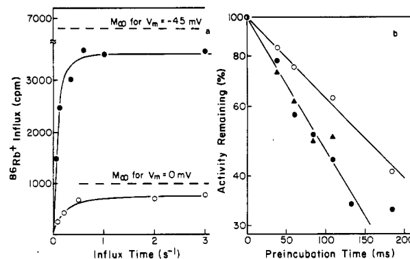
FIGURE 2: Activation and inactivation kinetics of acetylcholine receptor controlled flux of ^{86}\text{Rb}^+ into the membrane vesicles prepared from E. electricus electroplax, in the presence of a transmembrane voltage, pH 7.0, 1 ^{\circ}\text{C} . (a) Acetylcholine- (60 \mu\text{M} ) induced ^{86}\text{Rb}^+ influx in the presence (●) and absence (○) of a transmembrane voltage ( V_m = -45 mV). The lines were drawn by using the values of J_A and \alpha calculated from eq 3 of Table I in the preceding paper (Experimental Procedures): for V_m = -45 mV, J_A f_i = 5.1 \text{ s}^{-1} and \alpha = 7.0 \text{ s}^{-1} ; for V_m = 0 mV, J_A = 3.3 \text{ s}^{-1} and \alpha = 2.3 \text{ s}^{-1} . (b) Inactivation of acetylcholine-induced ^{86}\text{Rb}^+ influx in the presence (●, ▲) and absence (○) of a transmembrane voltage ( V_m = -45 mV): (○) preincubated with 1 mM acetylcholine, V_m = 0 mV ( \alpha = 5.5 ); (▲ and ●) preincubated with 1 and 5 mM acetylcholine, respectively, V_m = -45 mV ( \alpha = 8 \text{ s}^{-1} ). It should be noted that 1 and 5 mM acetylcholine gave the same inactivation rate coefficient in the presence of a transmembrane voltage. One volume of the membrane vesicles (1.6 mg of protein/mL) equilibrated with buffer A was mixed with 9.5 volumes of either buffer A or isotonic arginine solution containing various concentrations of acetylcholine. After various lengths of time, the activity was assayed in the second incubation of 1.5 s with ^{86}\text{Rb}^+ (40 \mu\text{Ci/mL} ) and 1 or 5 mM acetylcholine. The value of \alpha was calculated from \ln([M_\infty - (M_t)_T]/M_\infty)/\ln([M_\infty - (M_t)_{T=0}]/M_\infty) = e^{-\alpha T} . The activity remaining is indicated on the left side of the equation (Aoshima et al., 1981). (M_t)_T represents the radioactivity inside the vesicles when influx was measured for time t (1.5 s) after various preincubation times ( T ). (M_t)_{T=0} and M_\infty are the radioactivity inside the vesicles at time t (1.5 s) and at equilibrium, respectively.
