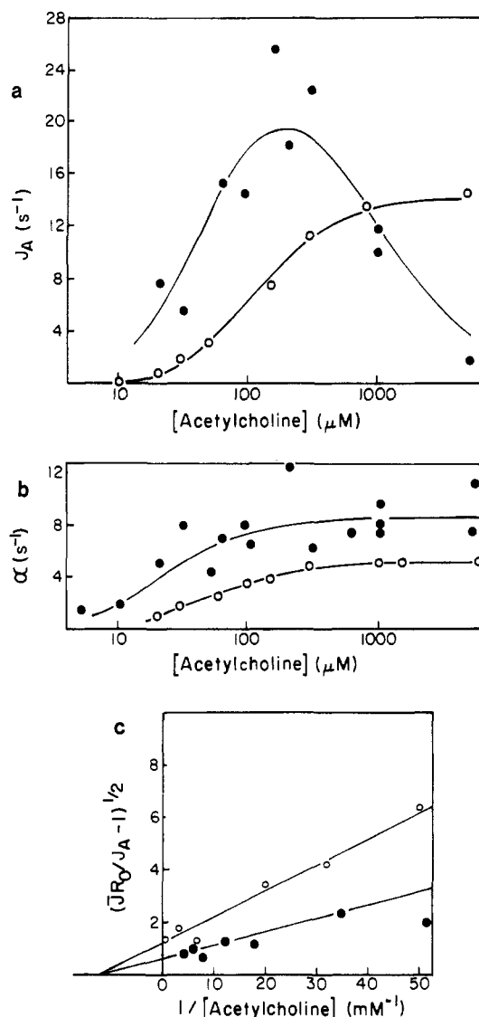
FIGURE 3: Effects of a transmembrane voltage on functioning of acetylcholine receptor from E. electricus electroplax. (a) Effect of a transmembrane voltage ( -45 mV) on the dependence of the influx rate coefficient, J_A , on acetylcholine concentration. One volume of the membrane vesicles equilibrated with buffer A (see Experimental Procedures) was mixed with 9.5 volumes of isotonic arginine solution containing ^{86}\text{Rb}^+ ( 40 \mu\text{Ci}/\text{mL} ) and various concentrations of acetylcholine. After various lengths of incubation time, the reaction was quenched by adding 5 volumes of d -tubocurarine ( 20 \text{ mM} ) in a buffer solution ( 11.1 \text{ mM NaCl} , 81 \text{ mM arginine chloride} , 1 \text{ mM CaCl}_2 , 1.5 \text{ mM sodium phosphate} , \text{pH } 7.0 ). An example of the measurement of the acetylcholine-induced ^{86}\text{Rb}^+ influx is shown in Figure 2a. For control experiments ( V_m = 0 \text{ mV} ), the vesicles were diluted with buffer A containing ^{86}\text{Rb}^+ and acetylcholine. The values of J_A in the presence (●) and absence (○) of the transmembrane voltage were calculated from the integrated rate equation (eq 3, Table I of the preceding paper) and normalized to each other by using a factor, f_i , of 0.33 at -45 \text{ mV} , \text{pH } 7.0 , 1^\circ\text{C} (eq 2). The points were obtained experimentally, and the lines in the absence and presence of the transmembrane voltage were calculated from eq 1a-I and 1-II, respectively, of Table I in the preceding paper by using the equilibrium constants listed in (c) and K_R = 800 \mu\text{M} . (b) Effect of a transmembrane voltage ( V_m = -45 \text{ mV} ) on the dependence of the inactivation rate coefficient, \alpha , on acetylcholine concentration: (○) V_m = 0 \text{ mV} ; (●) V_m = -45 \text{ mV} . (c) A linear plot of the relationship between the influx rate coefficient, J_A , and acetylcholine concentration, L : (○) V_m = 0 \text{ mV} ; (●) V_m = -45 \text{ mV} . Data from (a) were replotted by using eq 1b-I (Table I of preceding paper), neglecting the effect of inhibition at low acetylcholine concentrations ( 20 – 300 \mu\text{M} ). This procedure would give the maximum possible value of \Phi in the presence of a voltage. When V_m = 0 \text{ mV} , K_1 = 80 \pm 2 \mu\text{M} , 1/\Phi = 0.7 , J_A(\text{max}) = 15 \text{ s}^{-1} , and \bar{J} = 3 \times 10^7 \text{ M}^{-1} \text{ s}^{-1} . When V_m = -45 \text{ mV} , K_1 = 75 \pm 15 \mu\text{M} , 1/\Phi = 2.5 , J_A(\text{max}) = 26 \text{ s}^{-1} , and \bar{J} = 3 \times 10^7 \text{ M}^{-1} \text{ s}^{-1} .
